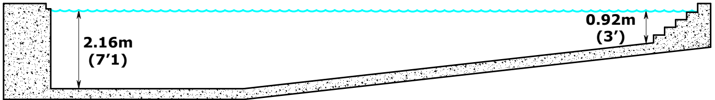
Section View
