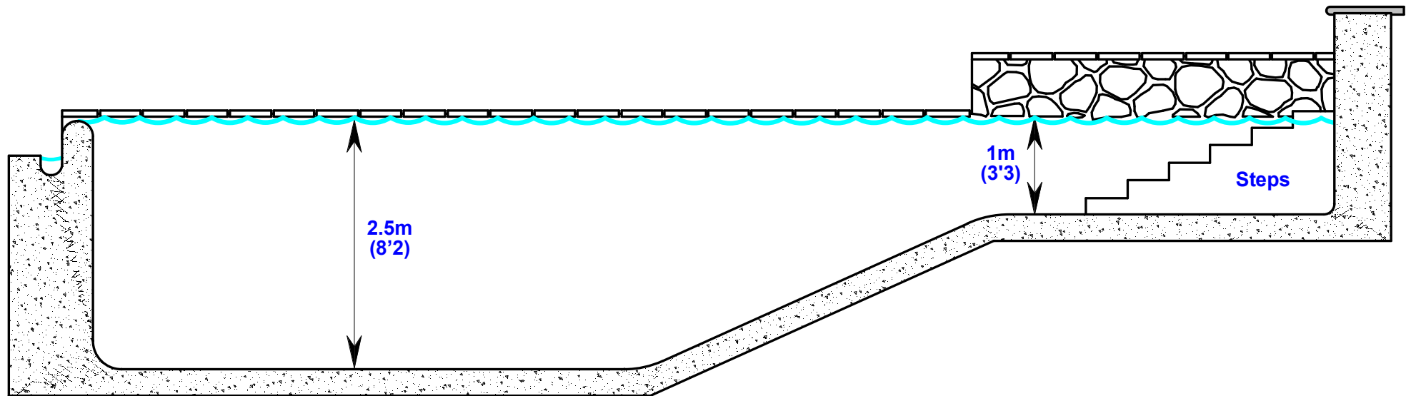
Section View
